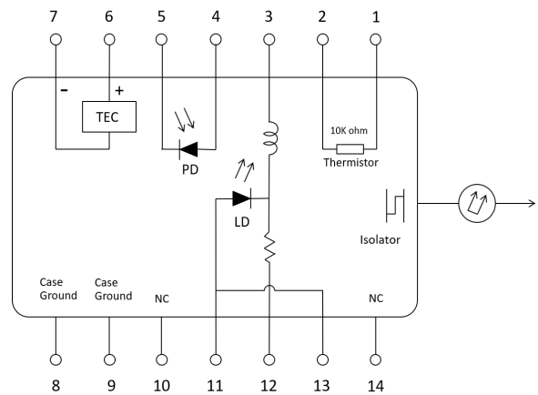
Fig. 4 Standard "Pinout 10" option
