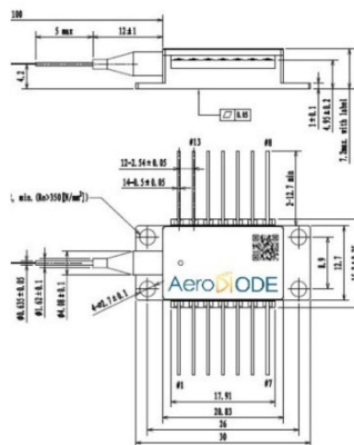
Dimensions are in mm
