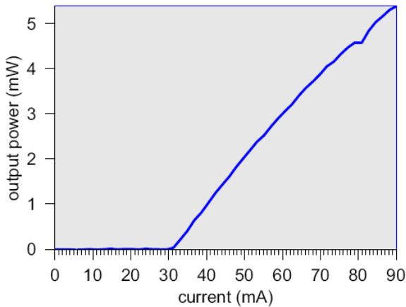
Current-Output-Power
