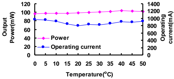
Power & Operating current vs Temperature
